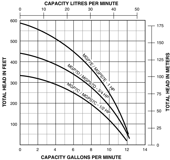
PUMP PERFORMANCE – 7 GPM
